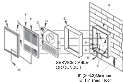
FIG. 2 SURFACE MOUNT
